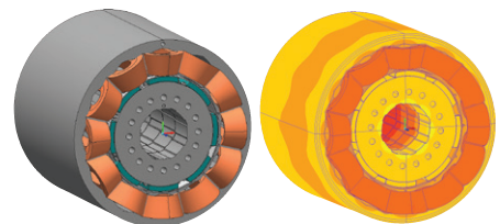
Coupled thermal analysis
