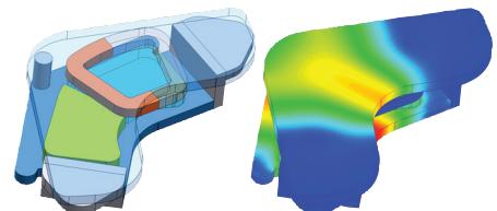
Voice coil actuator
