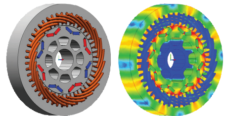
Traction motor
